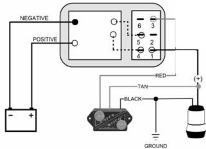
3 position switch diagram
