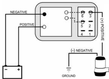
2 position switch diagram
