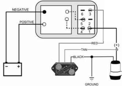
3 position switch diagram
